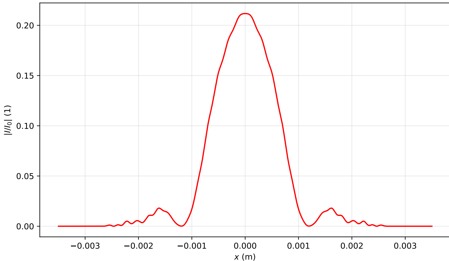
Intensity profile I(x, y = 0, z = 1.274)/I_0 , P_{in}=2.0P_{cr} , artificial time
